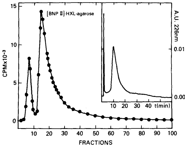
Fig. 2. Elution profiles for commercial [^3\text{H}] AVP on [BNP II]-HXL-agarose. The column (100 mm \times 10 mm I.D.) was equilibrated and eluted with 0.4 M sodium acetate, pH 5.7, at room temperature using a flow-rate of 1.0 ml/min. Samples containing 10 \mu\text{g} of [^3\text{H}] AVP were injected. Fractions of eighteen drops (810 \mu\text{l} ) collected directly into vials for scintillation counting. Inset: elution monitored on line by UV absorbance at 226 nm, 0.04 absorbance units (A.U.) full scale. V_0 = 2.5 ml.
